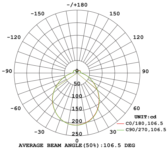
Light distribution
